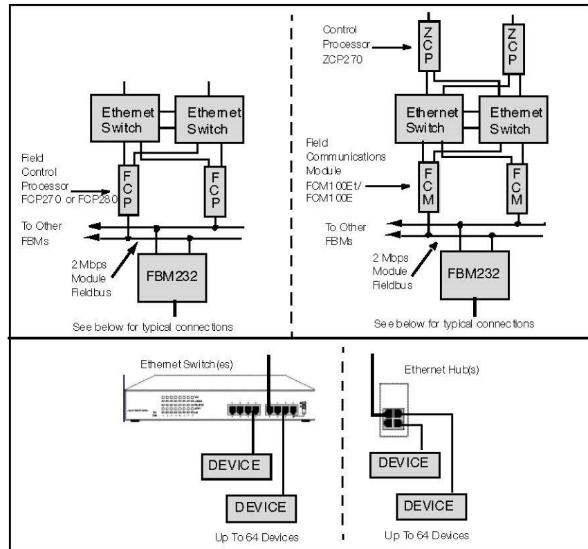
Figure 1. FBM232 in Typical Network Configuration
