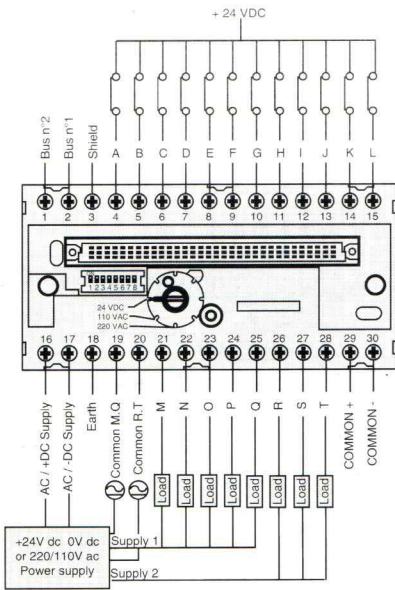
Type/Unit : CS20 - PCZB Central Unit
