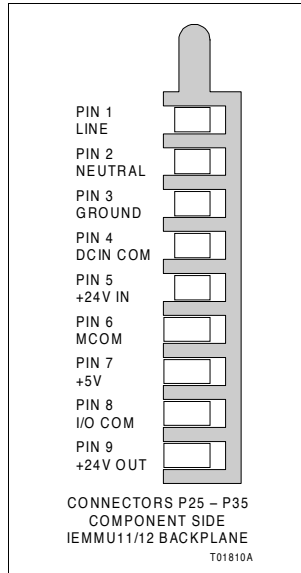
Figure 3-4. P25 - P35 Pin Location
