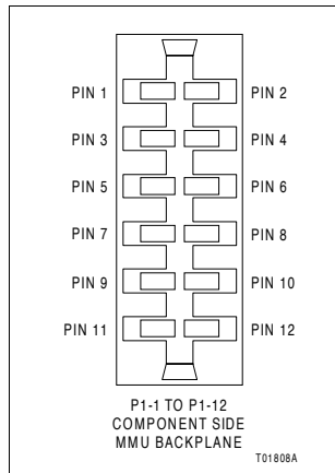
Figure 3-5. P1 Connector Pin Location
