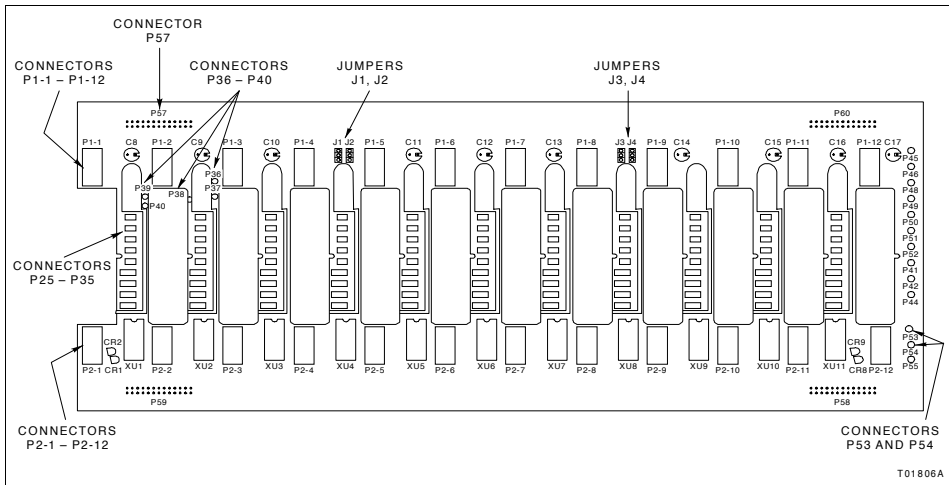
Figure 2-1. MMU Backplane Connector Locations (Module Side)
