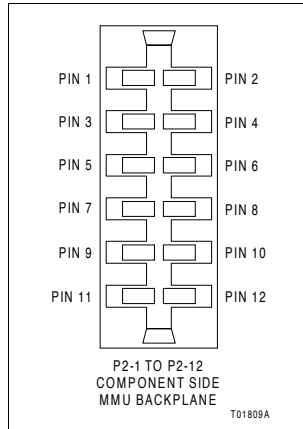
Figure 3-6. P2 Connector Pin Location
